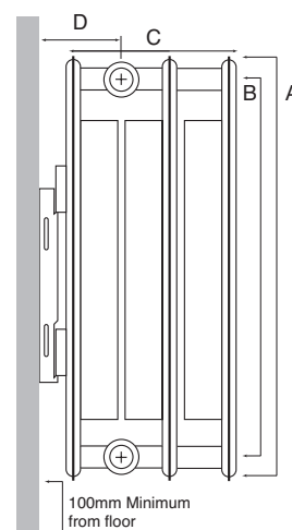
Triple Convector Type 33
