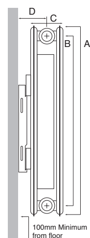
Double Panel Single Convector Type 21
